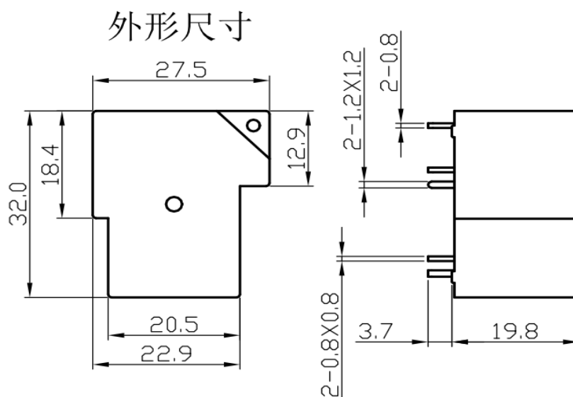
安装孔尺寸图/ Mounting dimension(bottom view)
